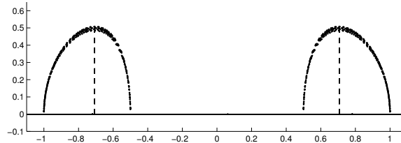
FIG. 6.1. Analogue of the circle theorem for the weight function of Example 4
