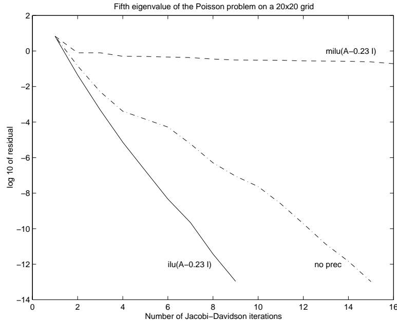
FIG. 5.1. The \log_{10} of the residual norm for iterative solves of the correction equations with 15 steps of GMRES without preconditioning (the dash-dotted curve: -\cdot ), with ILU preconditioner (the solid curve: - ), and with MILU preconditioner (the dashed curve: - - ). A is the 5-point discretized Poisson operator over a 20 by 20 grid. Both preconditioners are incomplete factorizations of A - \theta I with \theta = 0.23 . With this value of \theta we are aiming for the 5th smallest eigenvalue.
