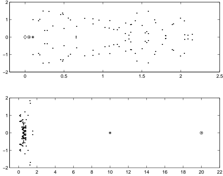
FIG. 4.1. The figures show the set of eigenvalues (the \cdot 's) of a normal matrix A (top figure), and of (A - \tau I)^{-1} (bottom figure). The diamond ( \diamond ) is the target value \tau ; the dotted circle ( \odot ) is the target eigenvalue, that is the eigenvalue closest to \tau in the upper figure, the absolute largest eigenvalue in the bottom figure. The asterisk ( * ) is the (harmonic) Ritz value.
