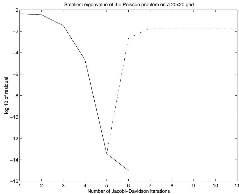
FIG. 5.2. The \log_{10} of the residual norm for direct solves of the correction equations with reorthogonalization (the solid curve: —) and without reorthogonalization (the dash-dotted curve: - ·). In the first part of the picture both curves coincide.
