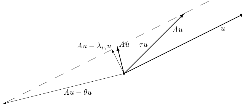
FIG. 4.2. The effect of testing with harmonic Ritz values when (\tau, u) approximates an eigenpair (\lambda_{i_0}, x_{i_0}) moderately well. The residual r = Au - \theta u is orthogonal with respect to the test subspace spanned by Au - \tau u . Note that |\lambda_{i_0} - \tau| \ll |\lambda_{i_0} - \theta| .
