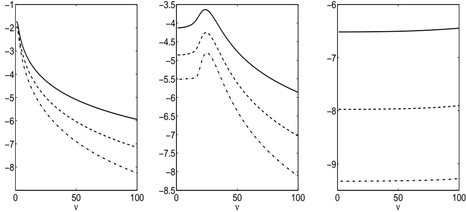
FIG. 4.1. Relative error (in \log_{10} scale) in the computation of the Bessel function K_\nu(\nu z) , using 3 terms (solid curve), 4 terms (dashed curve) and 5 terms (dashed-dotted curve) of the series involving Kummer U -functions. Left, \nu z = 1 + i , center \nu z = 10.1 + 20.5i and right \nu z = 100.1 + 120.5i .
